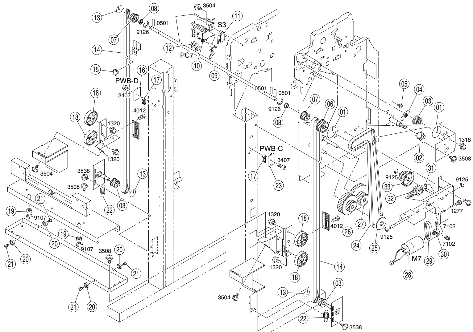
FIG. 4 ELEVATOR DRIVE
